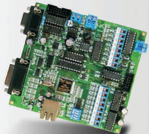
Easy PLC and Embedded PLC
