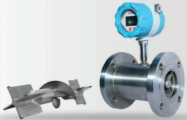
Helical rotor flow sensor and meter
