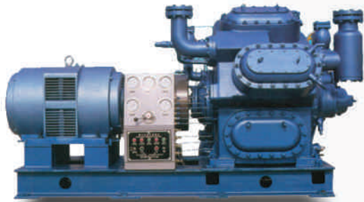
Ammonia Compressor Gas
